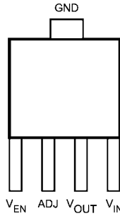
20126703 SOT-223, Top View LP38692MP-ADJ
